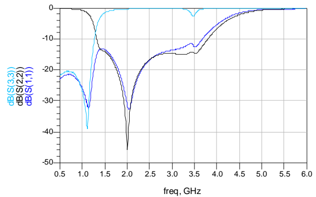
Return Loss
